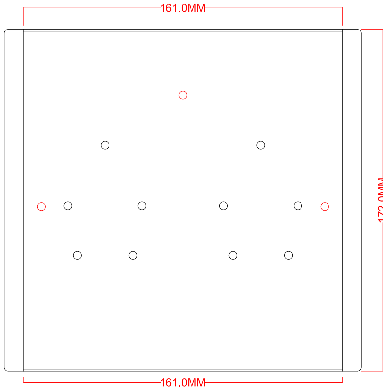
Bottom View
